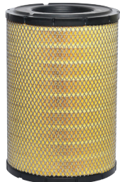
OEM NO. : 6I-2503 AUTOCOM NO: AIL-6I-2503 CAT (5558) SIZE(OD*ID*H) : 280*151*420mm
